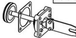
NO.201 Piston & Piston Rod Assy. 12,29,30,31,32,47,48,49,89
