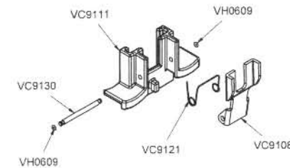
VC9112 ASSEMBLY
